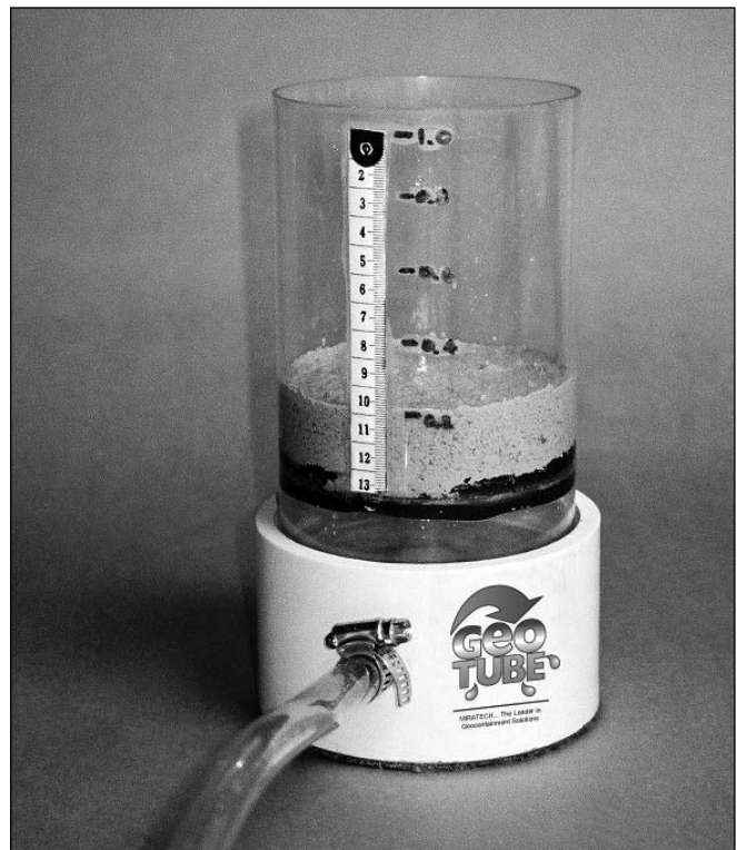
A Rapid Dewatering Test (RDT) unit was used to simulate filtration and dewatering.
