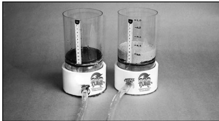
Numerous filter fabrics were tested in order to determine capture and filtrate quality. On the left, a RDT unit is displayed without tailings. On the right, the tailings are added on top of the Geotube® GT500 fabric.
